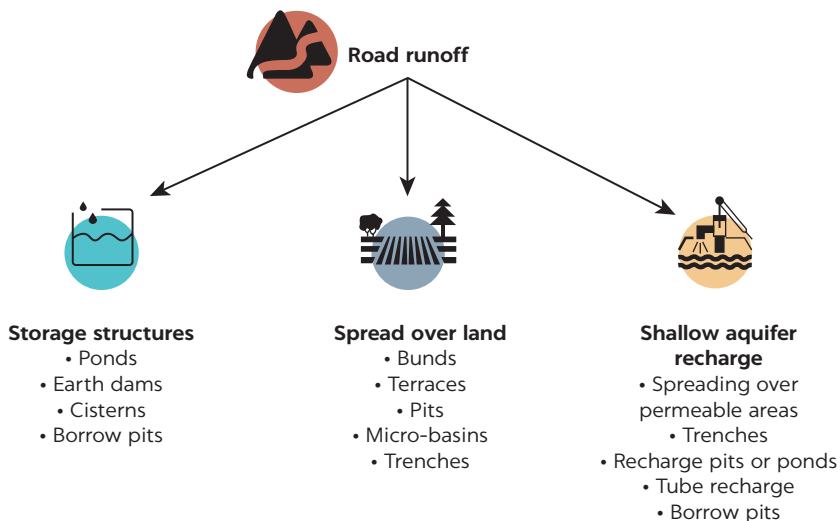
FIGURE 4.1 Water runoff
