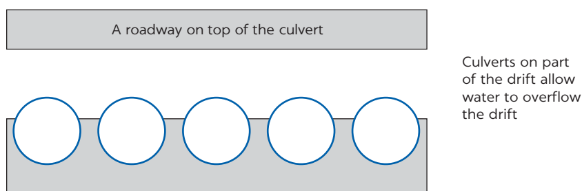
FIGURE 9.1 Sandwich drift to ensure passability
