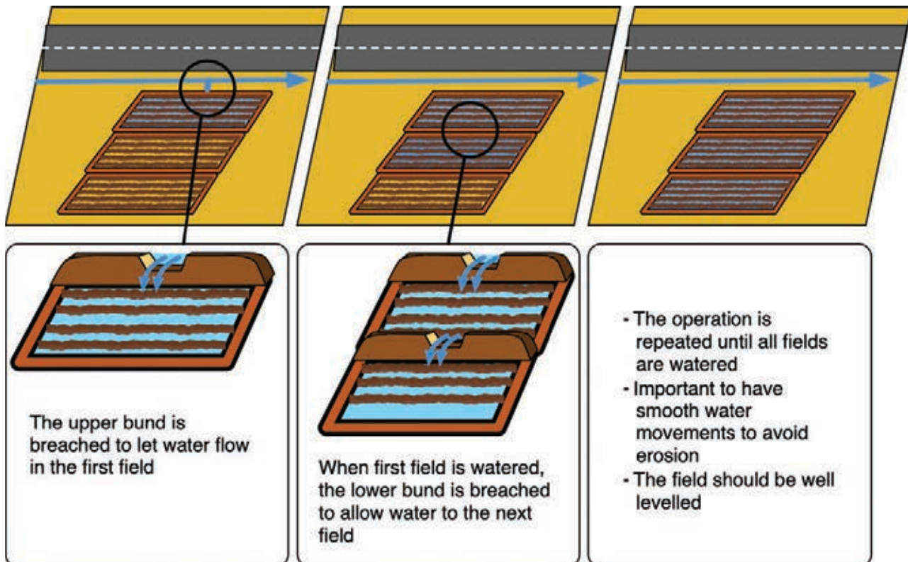
FIGURE 4.4 Cascading irrigation sequence
