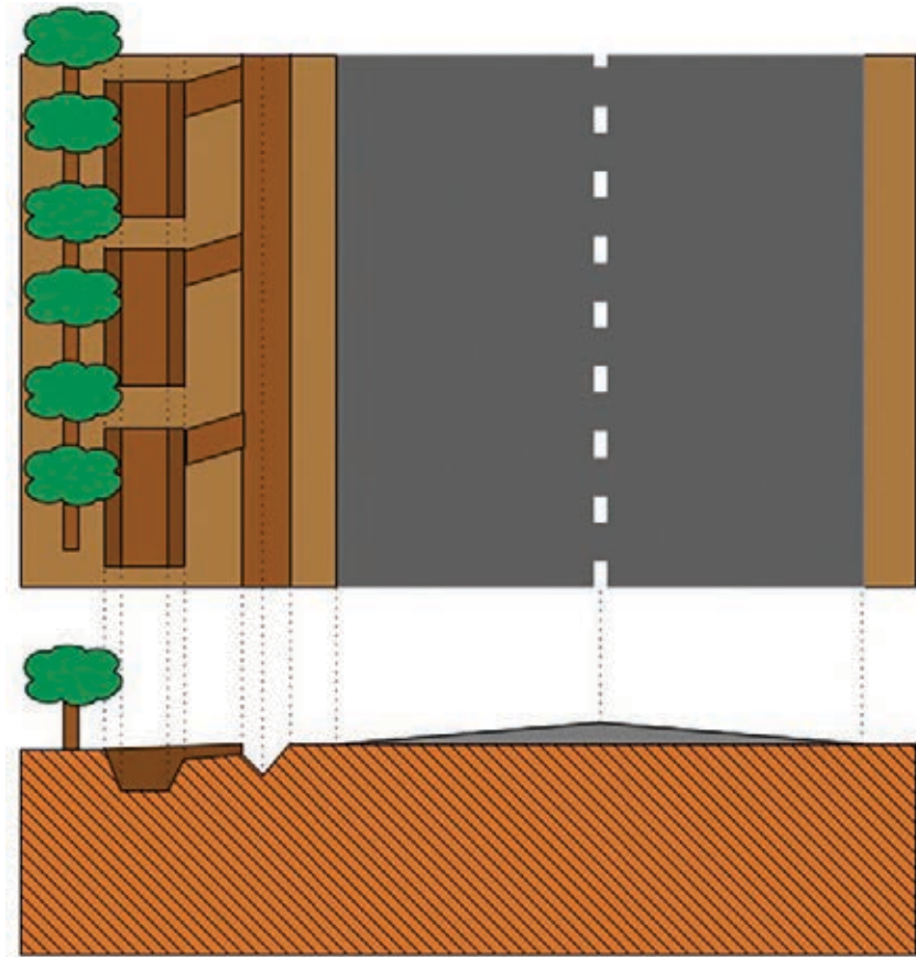
FIGURE 12.4 Infiltration trenches collecting road runoff to enhance the growth of seedlings
