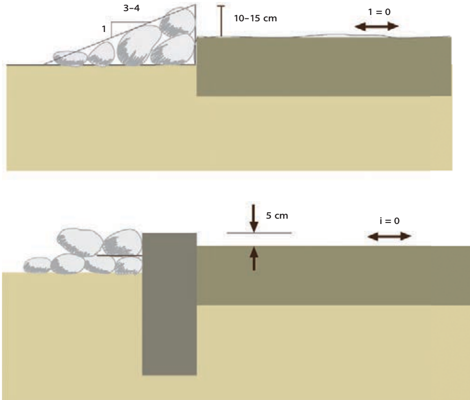
FIGURE 7.1 Submersible road criteria
