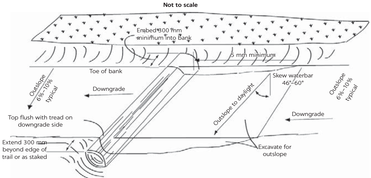
FIGURE 10.2 Rock water bar specifications
